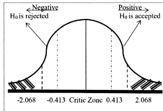
Figure 1: Hypothesis Testing of t_{test}
